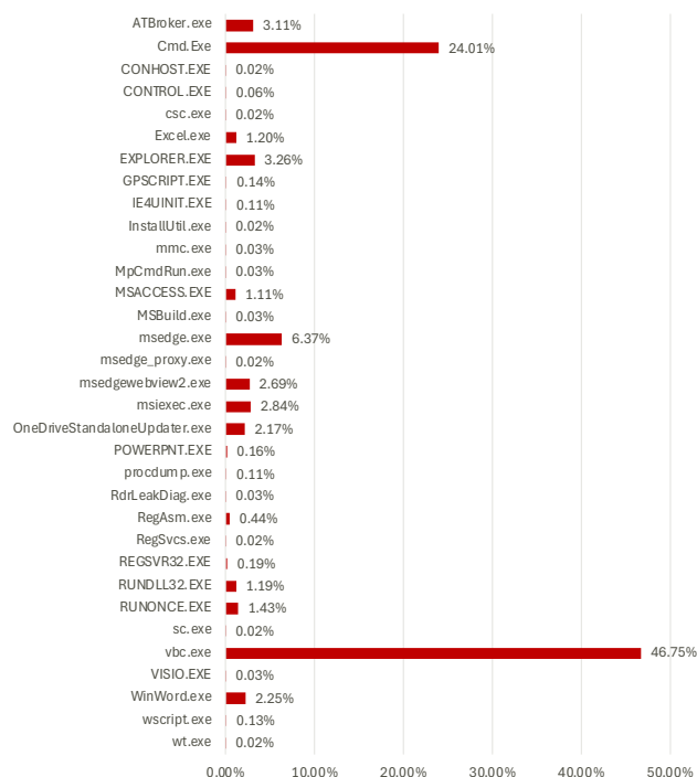
Figure 42. Q4 2024 Windows (LOLBAS) Detections
