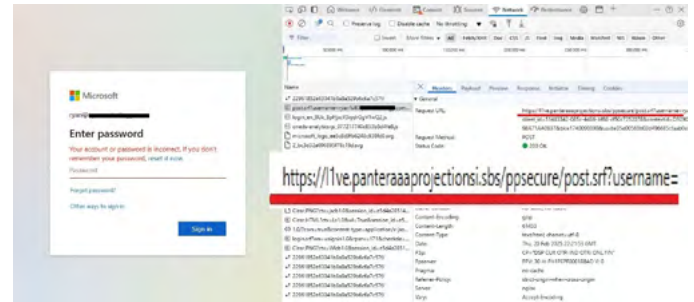
Figure 8. Phishing.3.header
