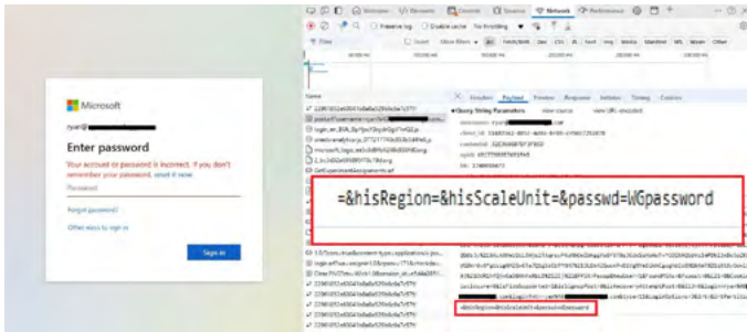
Figure 7. Phishing.3.human
