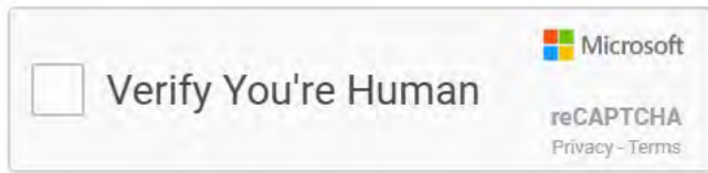
Figure 6. Phishing.3.human
