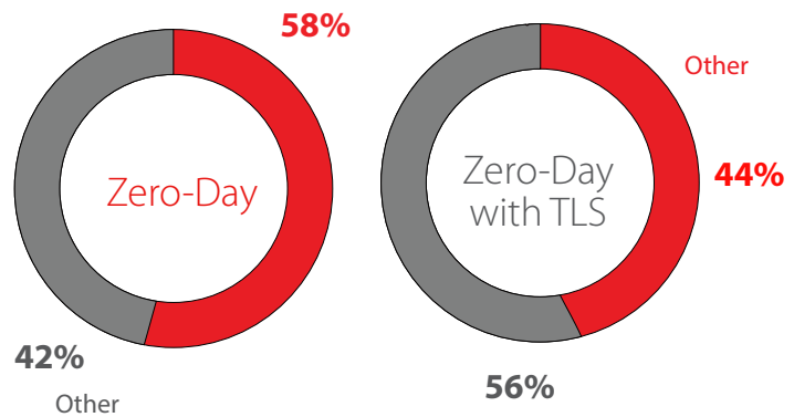
Figure 6. Zero-Day Malware
