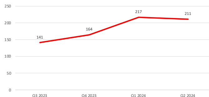
Figure 43. 2023-2024 Cryptominer Detections
