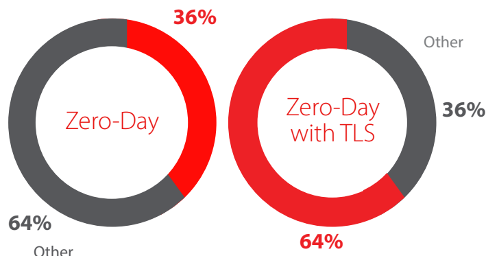
Figure 5. Zero-Day Malware
