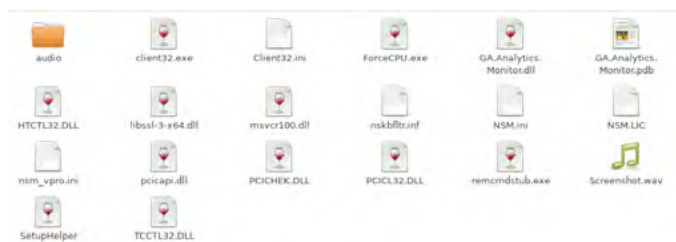
Figure 28. Extracted contents
