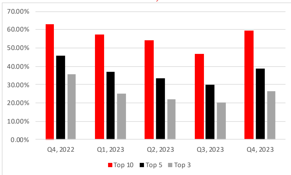
Figure 23. Total Share of Top Signatures by Volume Combined
