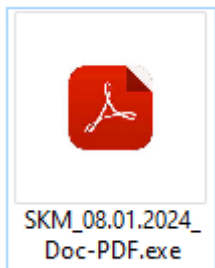
Figure 12. Zmutzy Icon
