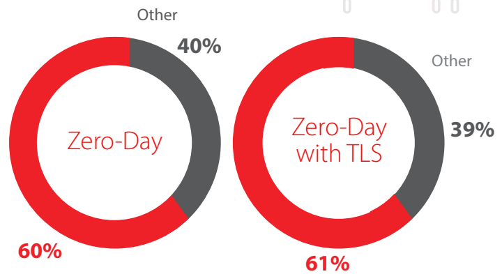
Figure 6. Zero-Day Malware
