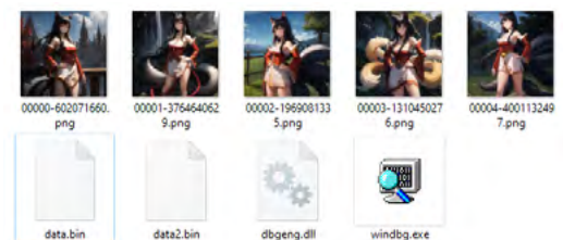
Figure 7. DarkGate
