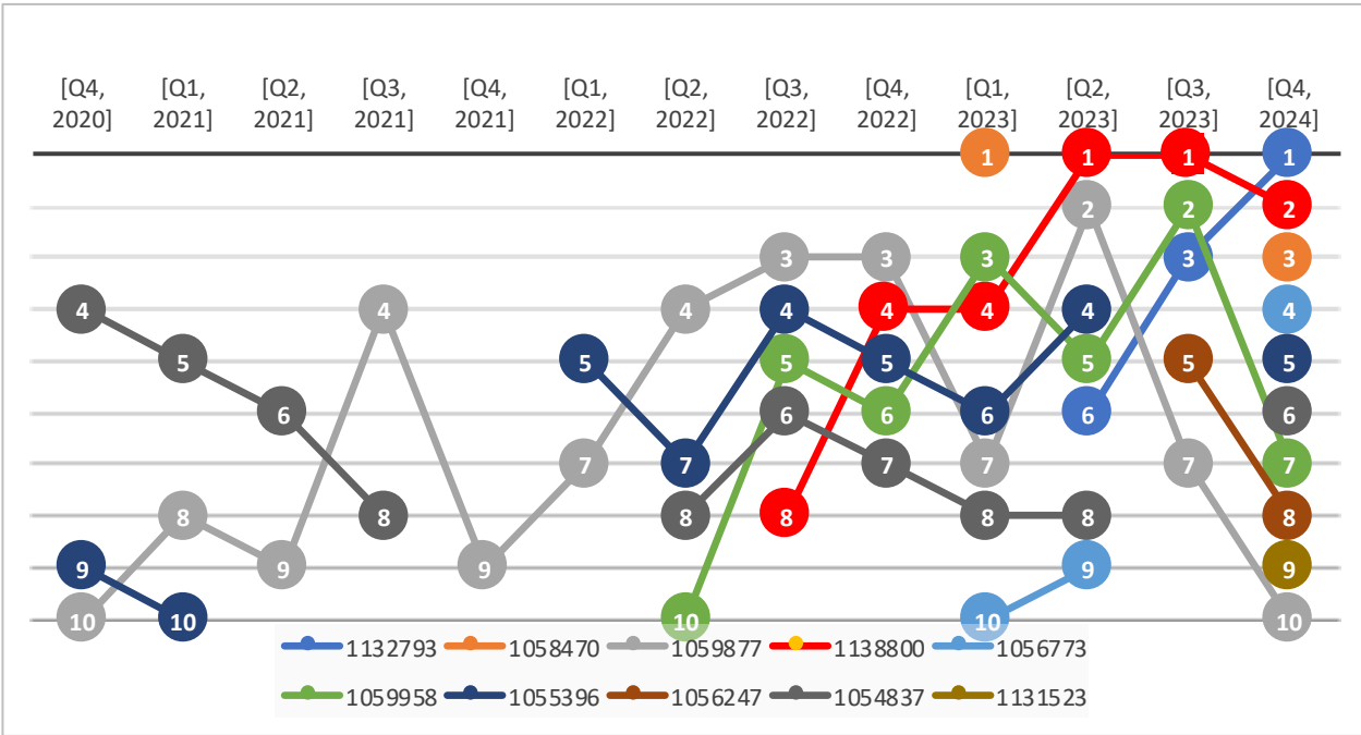
Figure 22. History of Prominent Signatures in the Top 10 Since Q2 2020
